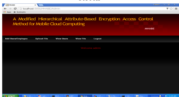
Fig.6: Admin Screen
